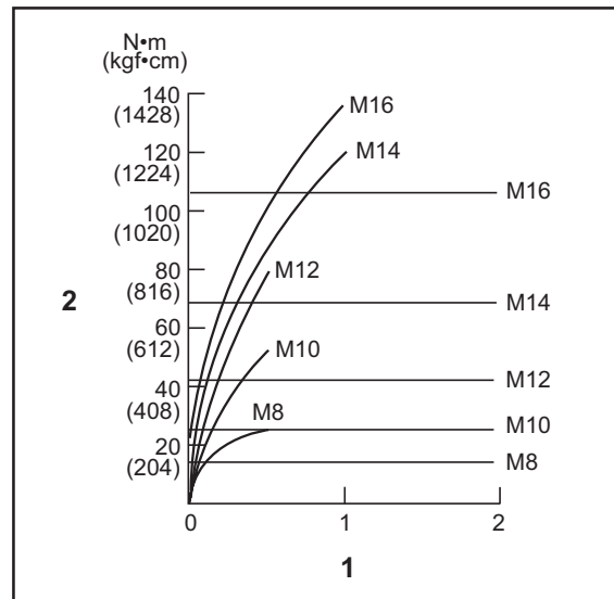
1. Fastening time (second) 2. Fastening torque
