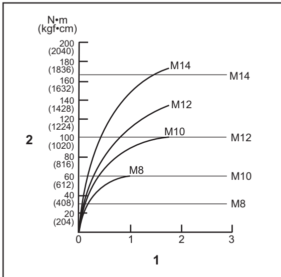
1. Fastening time (second) 2. Fastening torque
